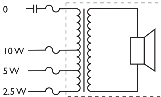
Circuit diagram
