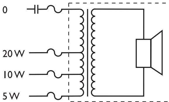
Circuit diagram
